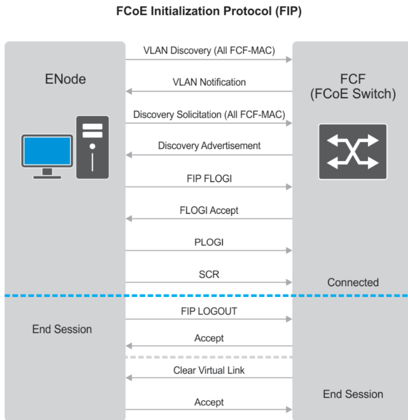
Figure 33. FIP Discovery and Login Between an ENode and an FCF
